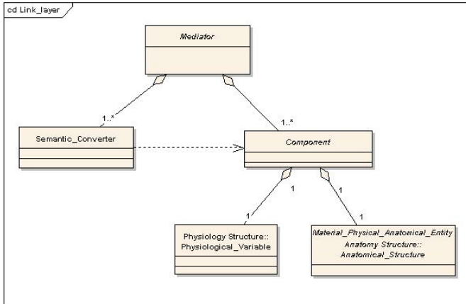
Figure 3. Design for the layer responsible of the information flow among the individual physiological models.
